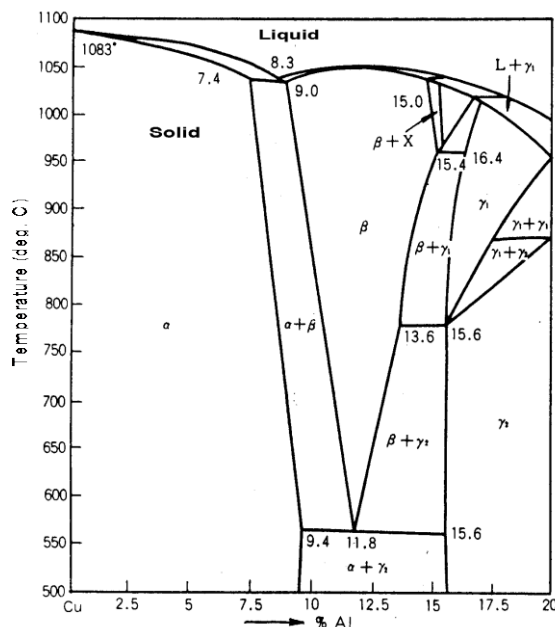
Figure 1.1 An equilibrium phase diagram of Cu-Al alloying system [Ref. 4]
