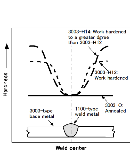
Figure 2.1 variations in weld hardness distribution of nonheat-treatable aluminum [Ref. 5]
