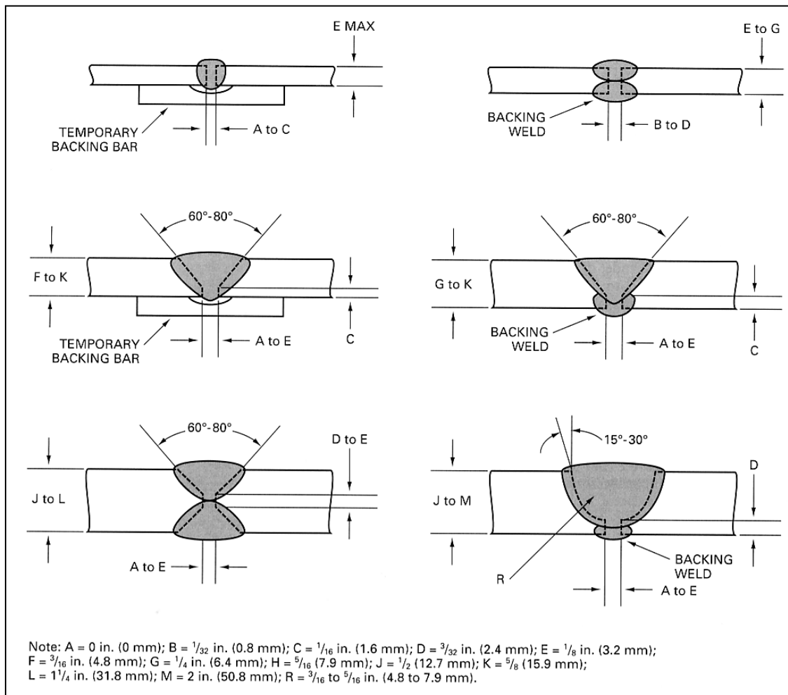
Figure 2.3 Suggested designs for arc-welded butt joints in nickel and nickel alloys [Ref. 2]
