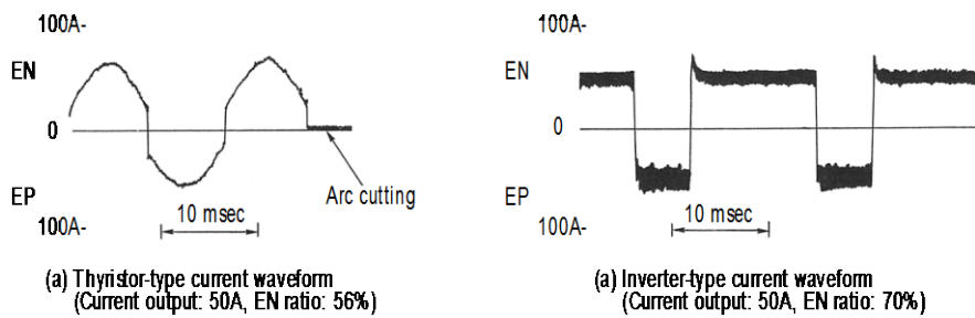
Figure 3.2 A comparison of output current waveforms of thyristor- and inverter-type power sources [Ref. 1]
